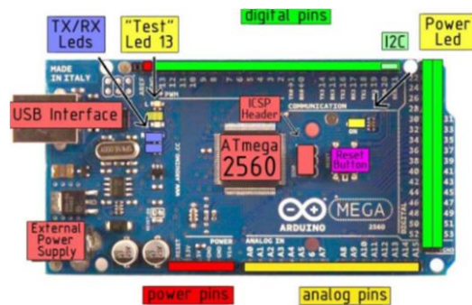
Fig.3 shows the Arduino MEGA Board
