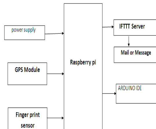
Fig.1 Block Diagram
